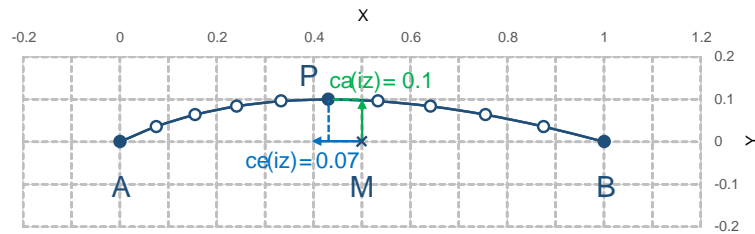
Figure J.4. With the expansion coefficient ce > 0 and the alignment coefficient ca > 0 , the method reconstitutes the points at intervals of expanding size ( ce ) along an arc with an alignment offset ( ca ) from the great circle between tie points A and B.
