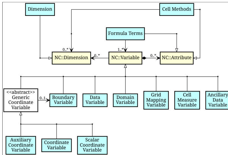
Figure I.1. The relationships between CF-netCDF elements and their corresponding netCDF variables, dimensions and attributes (identified here with the "NC" prefix). It is useful to define an abstract generic coordinate variable that can be used to refer to coordinates when their type (coordinate, auxiliary or scalar coordinate variable) is not an issue.
