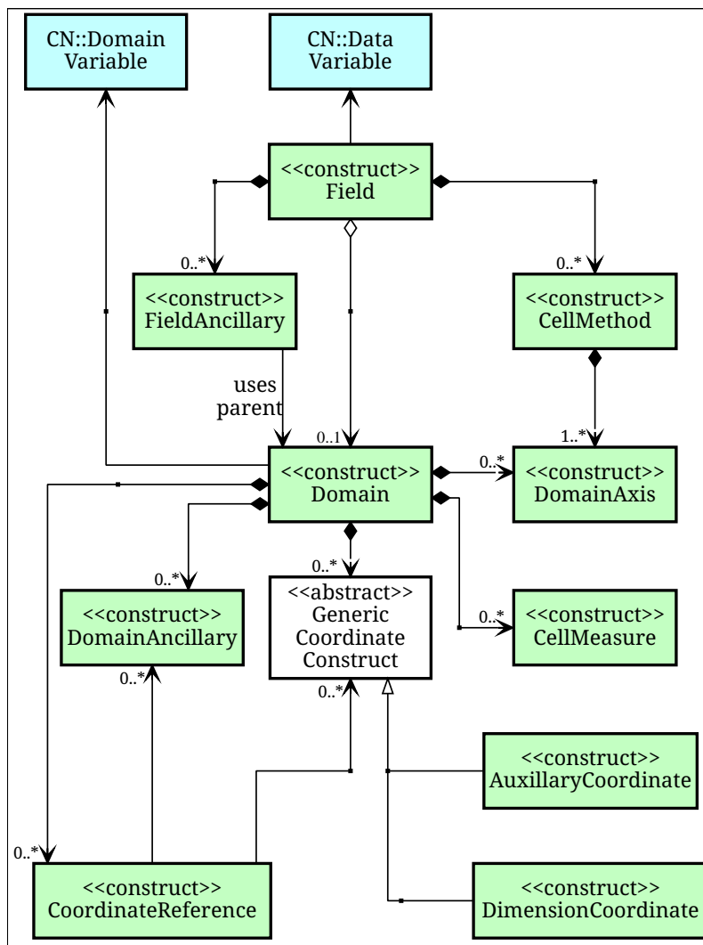
Figure I.2. The constructs of the CF data model. The field and domain constructs correspond to CF-netCDF data and domain variables respectively (defined in Figure I.1 and identified here with the "CN" prefix). Relationships between the other constructs and CF-netCDF are given in Figure I.3 and Figure I.4 . It is useful to define an abstract generic coordinate construct that can be used to refer to coordinates when their type (dimension or auxiliary coordinate construct) is not an issue.
