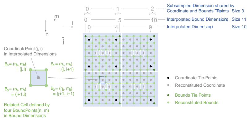
Figure 8.4. Example of 2D bounds interpolation showing the bounds tie points and reconstituted bound points within a continuous area consisting of four interpolation subareas. The dimensions are show for one of the two axes only. The index relationship between coordinate point indices and the related bound point indices is indicated.
